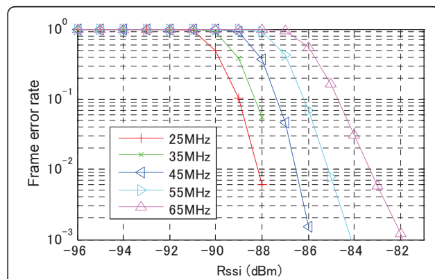
Figure 11 FER of SoftDec (2 bit A/D, \Delta = 1/4 ).
