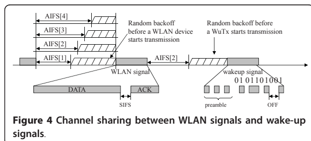
Figure 4 Channel sharing between WLAN signals and wake-up signals.
