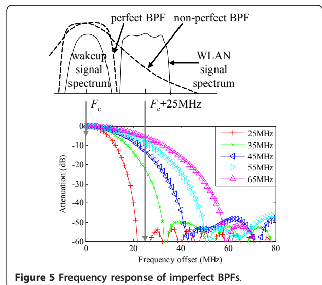
Figure 5 Frequency response of imperfect BPFs.
