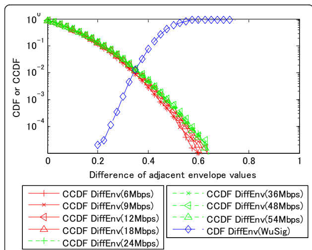
Figure 10 Distribution of difference of adjacent envelope samples (RSSI = -82 dBm, BPF bandwidth = 65 MHz).
